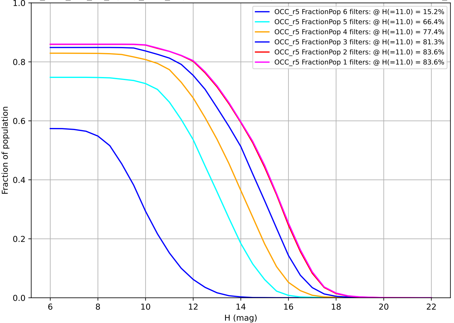
too_elab_r16_d2_ugrizy_v3.4_10yrs: Fraction of population with colors in X filters OCC_r5
