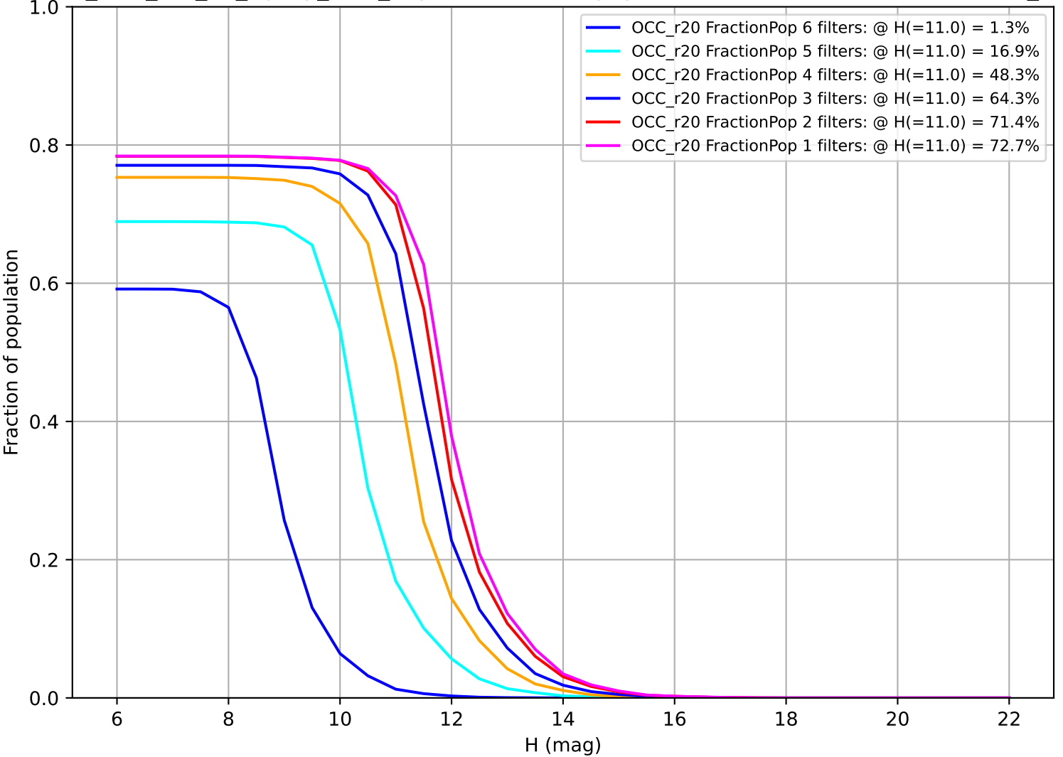
too_elab_r16_d2_ugrizy_v3.4_10yrs: Fraction of population with colors in X filters OCC_r20
