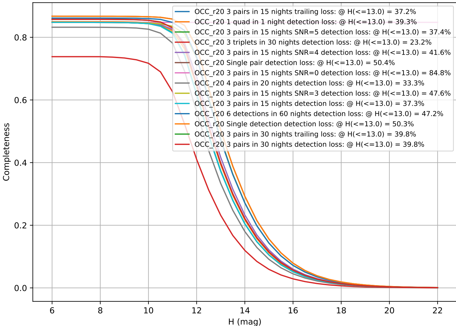
too_elab_r16_d2_ugrizy_v3.4_10yrs: CumulativeCompleteness
