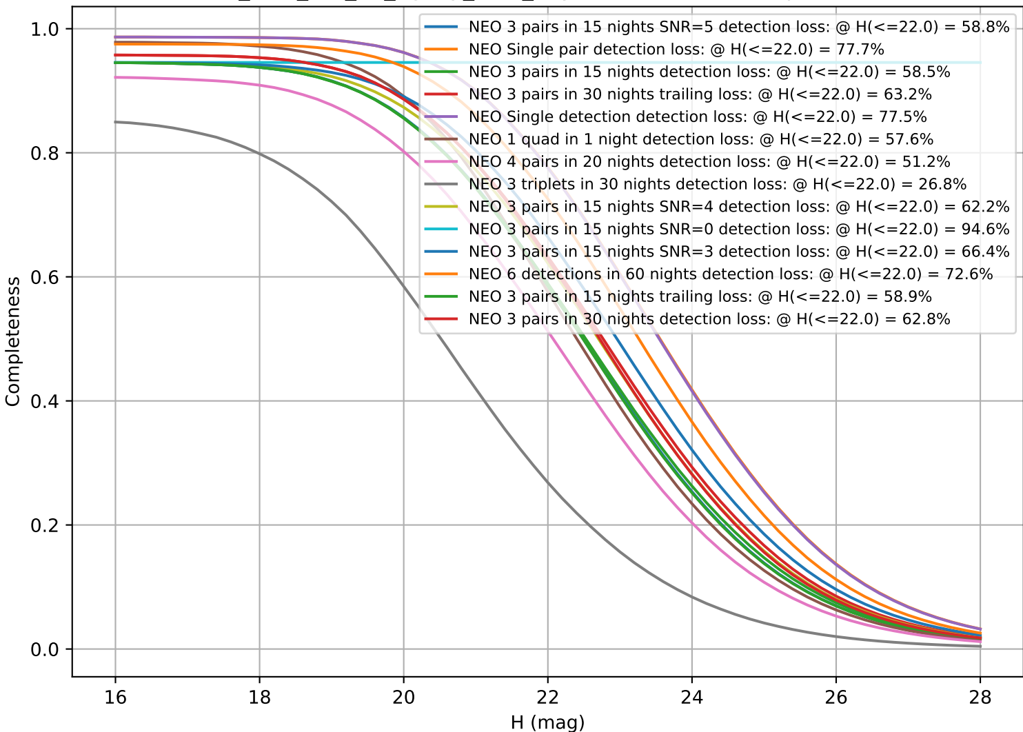
too_elab_r16_d2_ugrizy_v3.4_10yrs: CumulativeCompleteness
