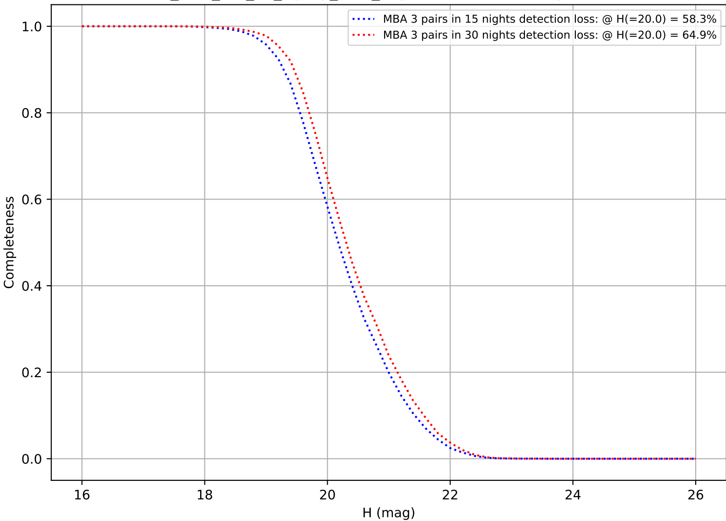
too_elab_r16_d2_ugrizy_v3.4_10yrs: DifferentialCompleteness
