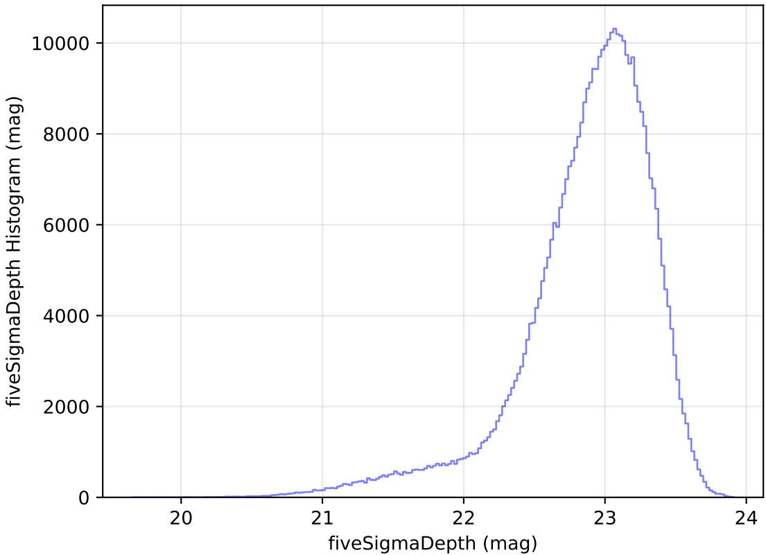
too_elab_r16_d2_ugrizy_v3.4_10yrs z: fiveSigmaDepth Histogram
