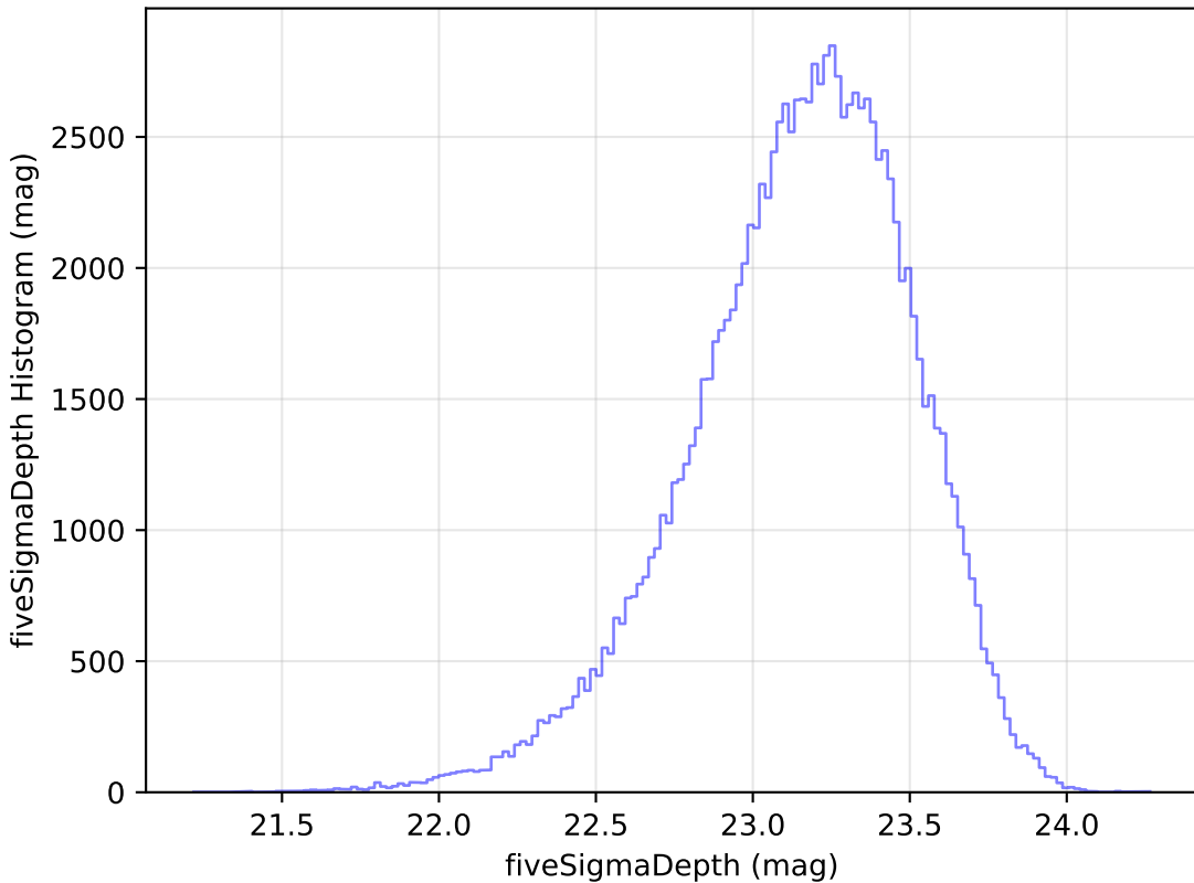
too_elab_r16_d2_ugrizy_v3.4_10yrs u: fiveSigmaDepth Histogram
