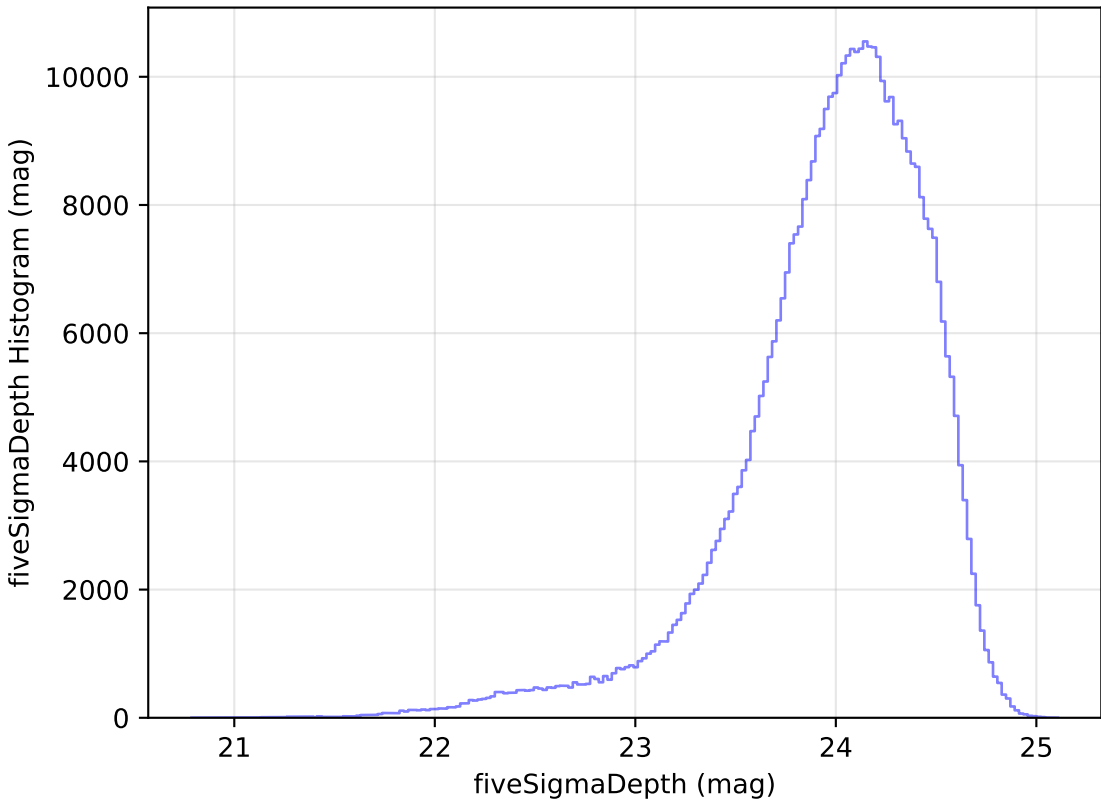
too_elab_r16_d2_ugrizy_v3.4_10yrs r: fiveSigmaDepth Histogram
