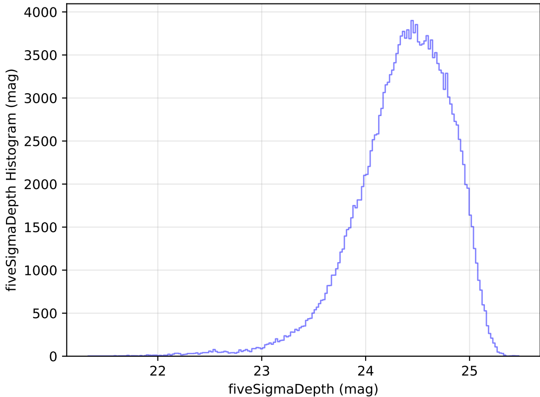
too_elab_r16_d2_ugrizy_v3.4_10yrs g: fiveSigmaDepth Histogram
