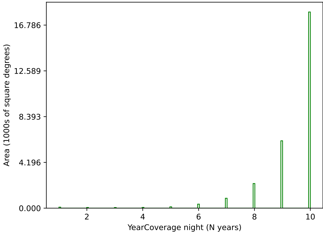
too_elab_r16_d2_ugrizy_v3.4_10yrs g band: YearCoverage night
