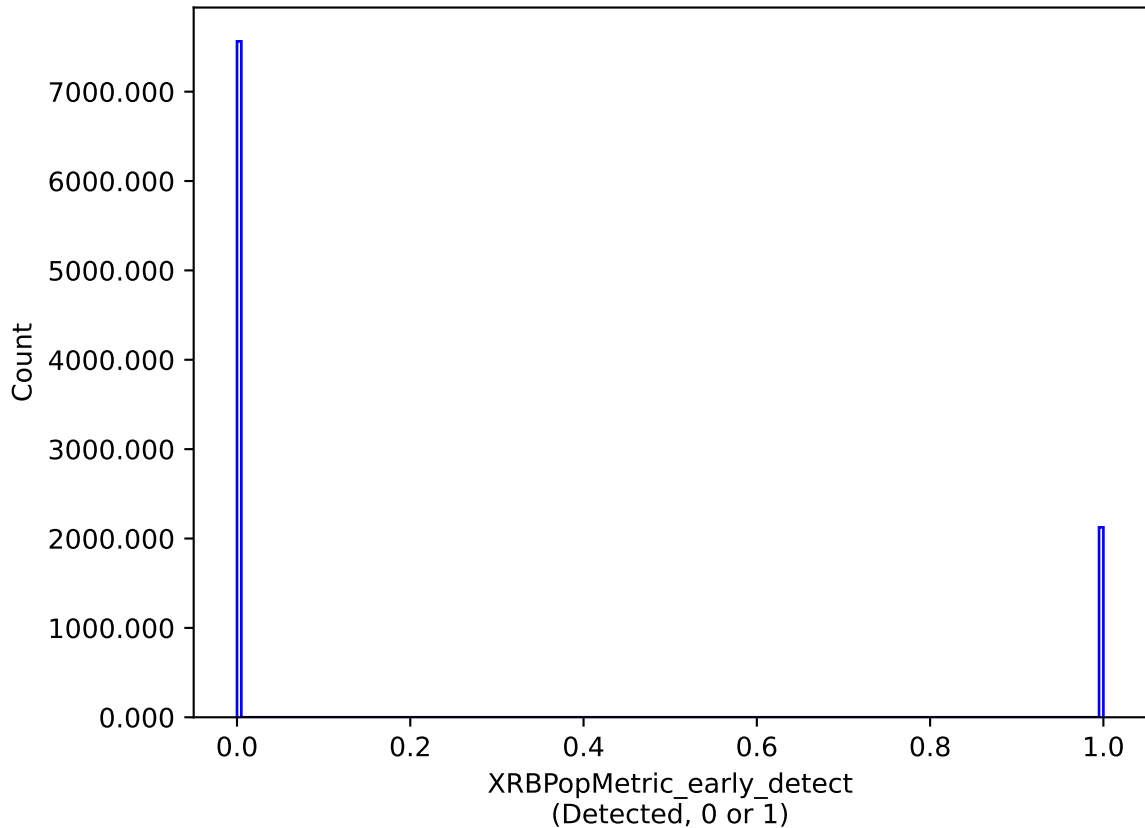
too_elab_r16_d2_ugrizy_v3.4_10yrs : XRBPopMetric_early_detect
