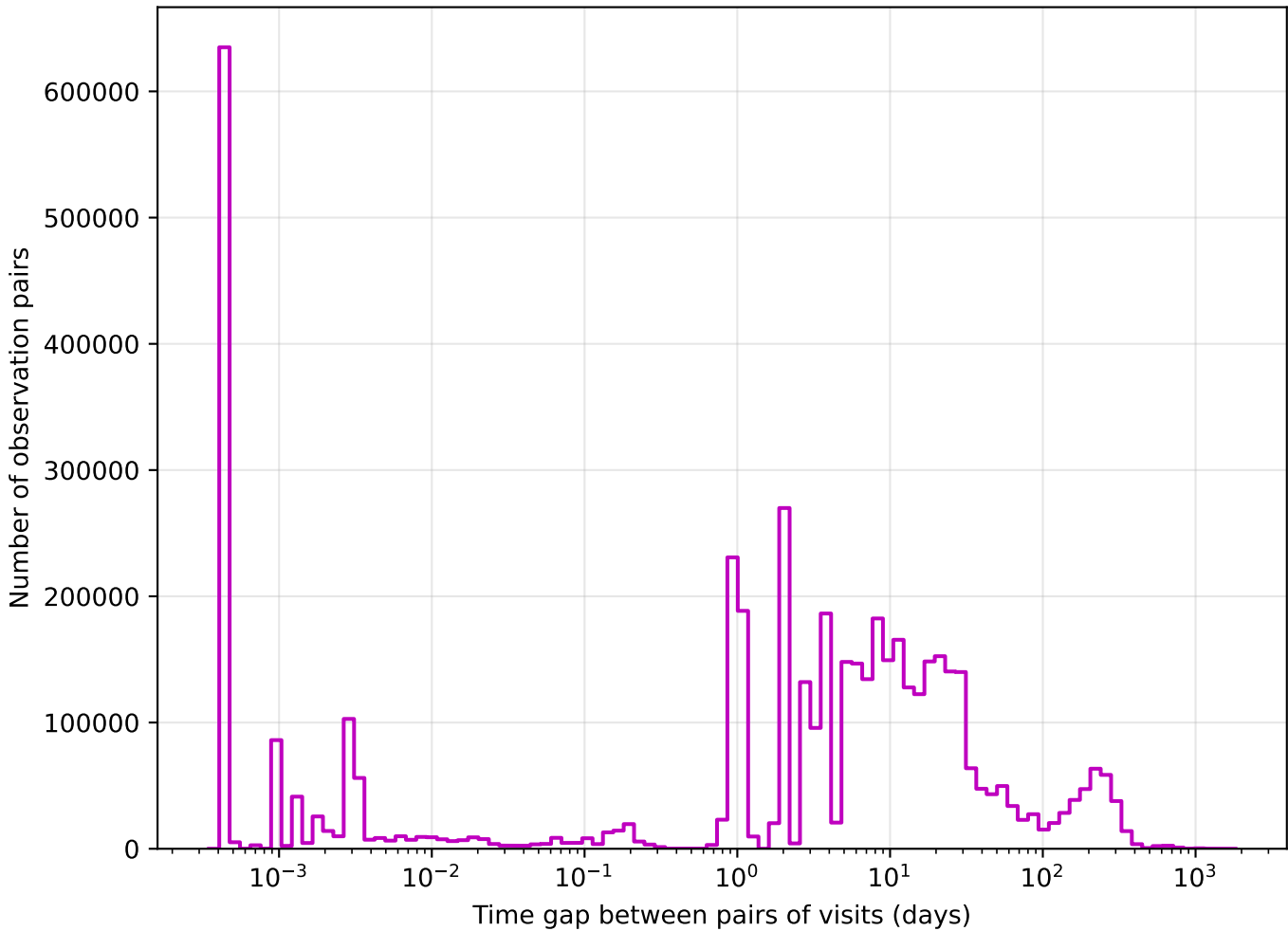
too_elab_r16_d2_ugrizy_v3.4_10yrs z band: Tgaps observationStartMJD
