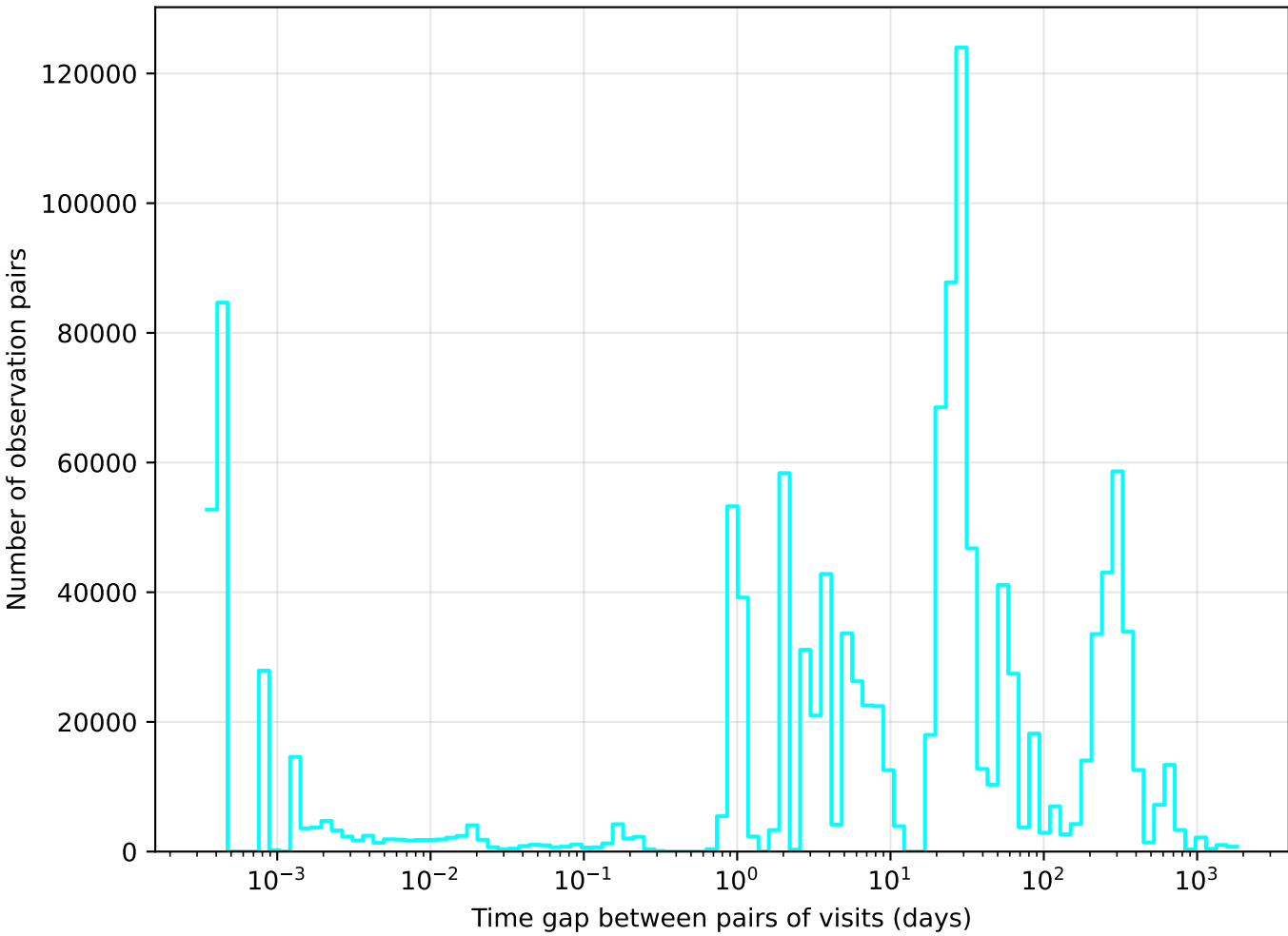
too_elab_r16_d2_ugrizy_v3.4_10yrs u band: Tgaps observationStartMJD
