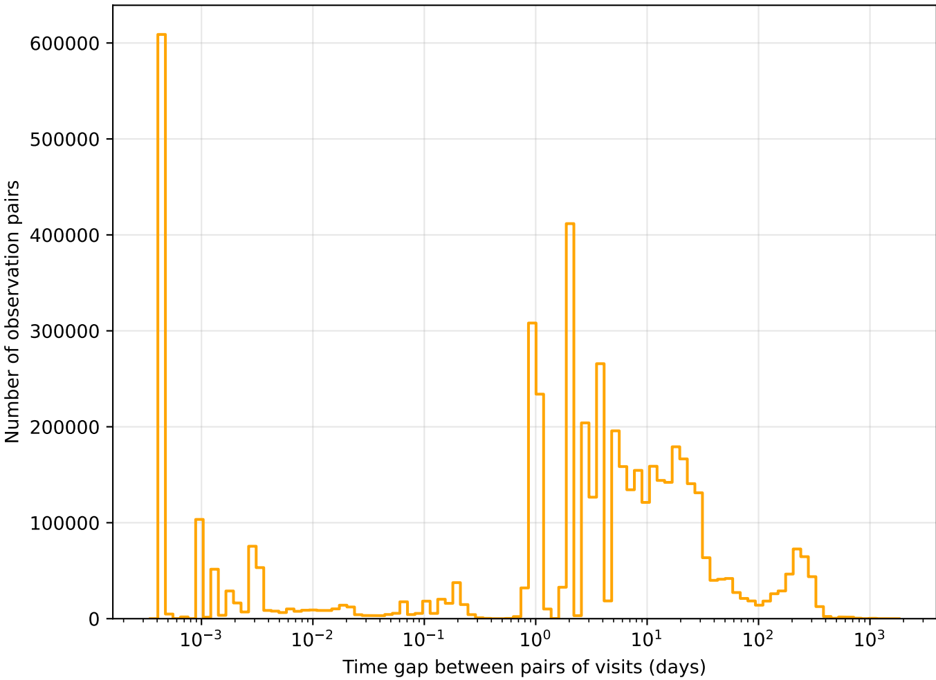
too_elab_r16_d2_ugrizy_v3.4_10yrs r band: Tgaps observationStartMJD
