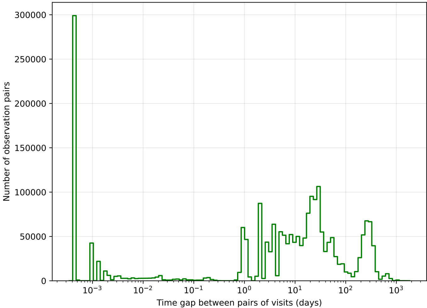
too_elab_r16_d2_ugrizy_v3.4_10yrs g band: Tgaps observationStartMJD
