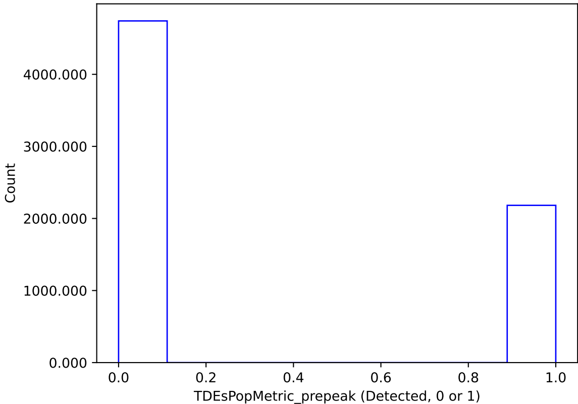
too_elab_r16_d2_ugrizy_v3.4_10yrs : TDEsPopMetric_prepeak
