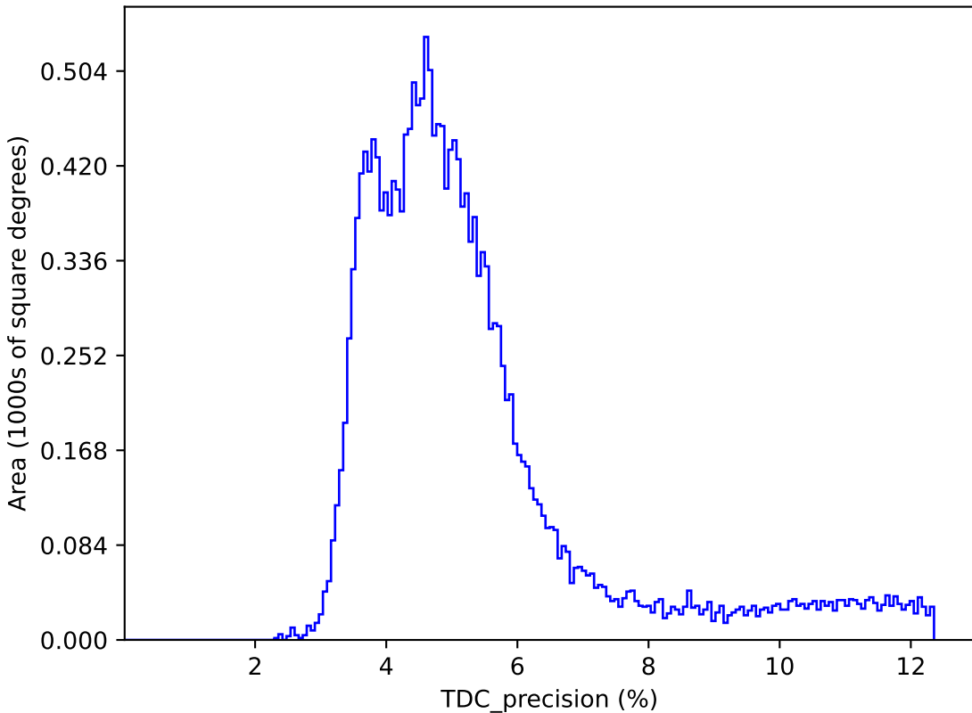
too_elab_r16_d2_ugrizy_v3.4_10yrs : TDC_precision
