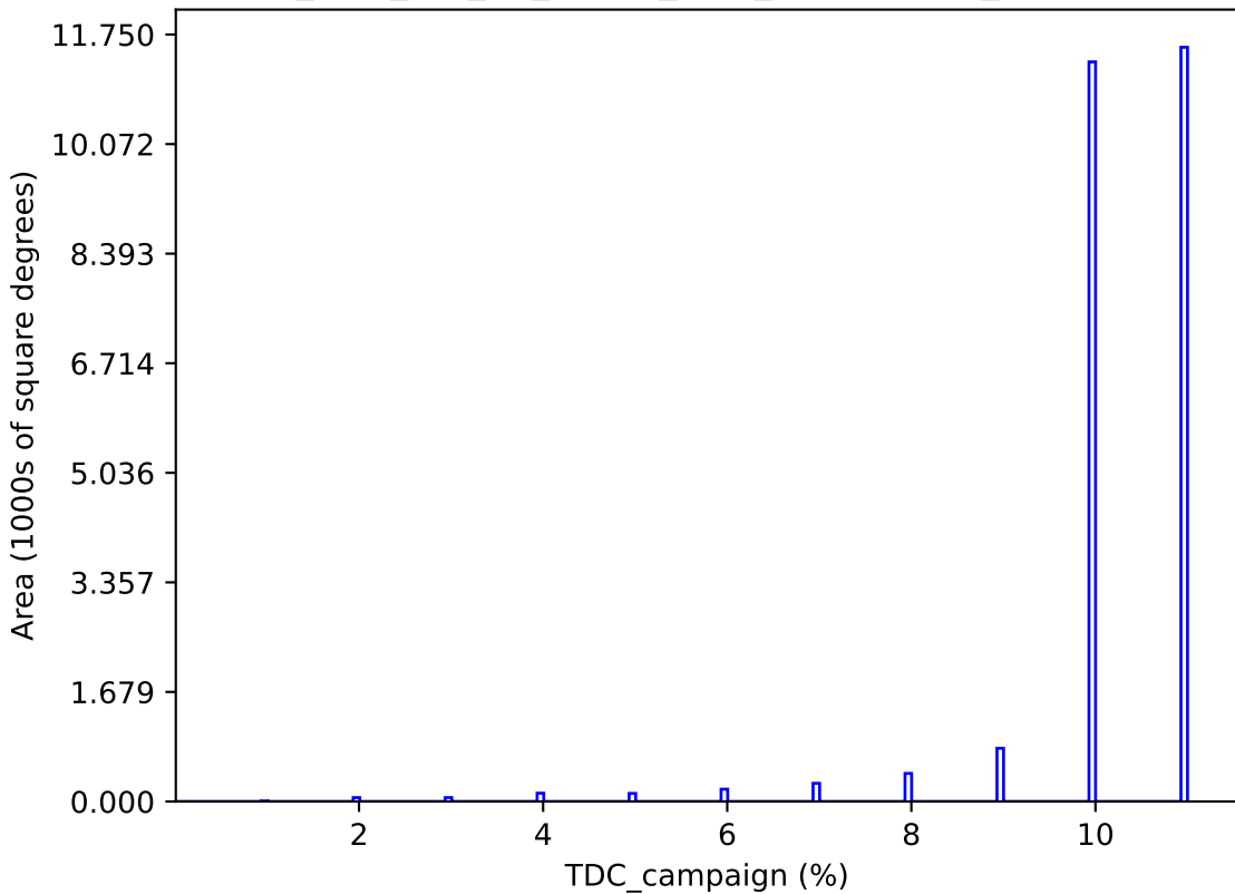
too_elab_r16_d2_ugrizy_v3.4_10yrs : TDC_campaign
