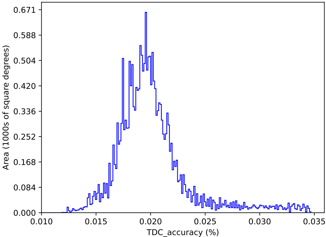
too_elab_r16_d2_ugrizy_v3.4_10yrs : TDC_accuracy
