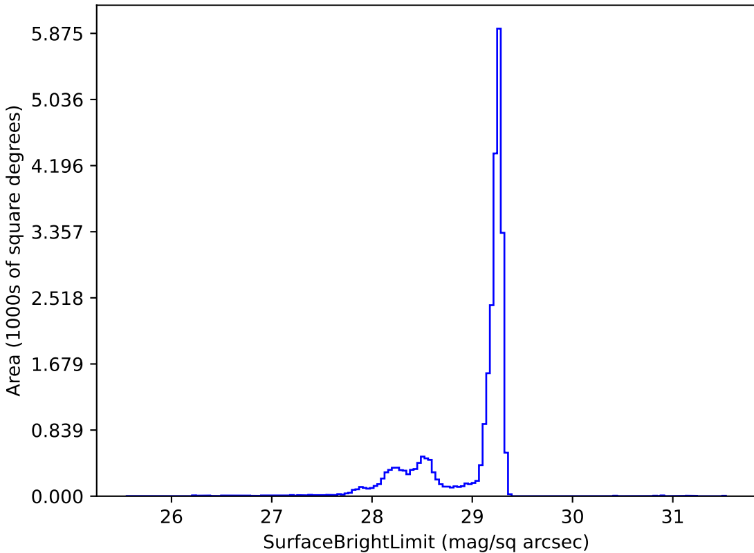
too_elab_r16_d2_ugrizy_v3.4_10yrs z: SurfaceBrightLimit
