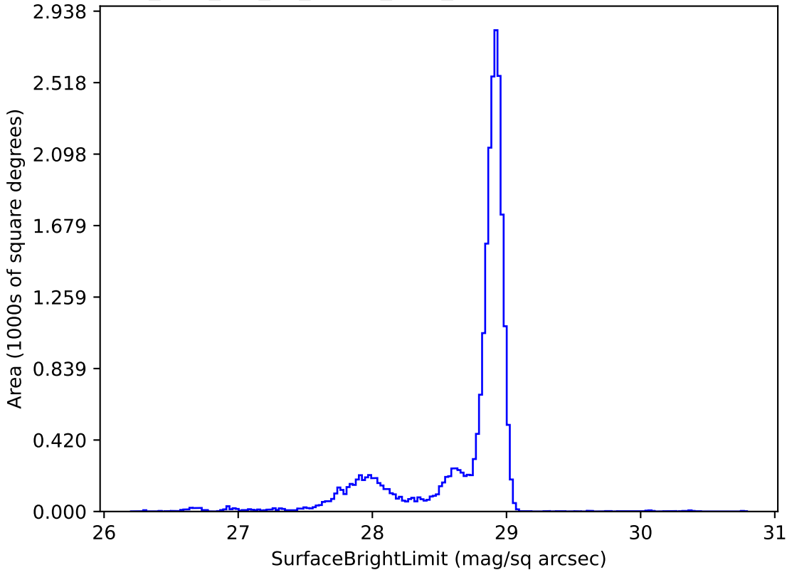
too_elab_r16_d2_ugrizy_v3.4_10yrs u: SurfaceBrightLimit
