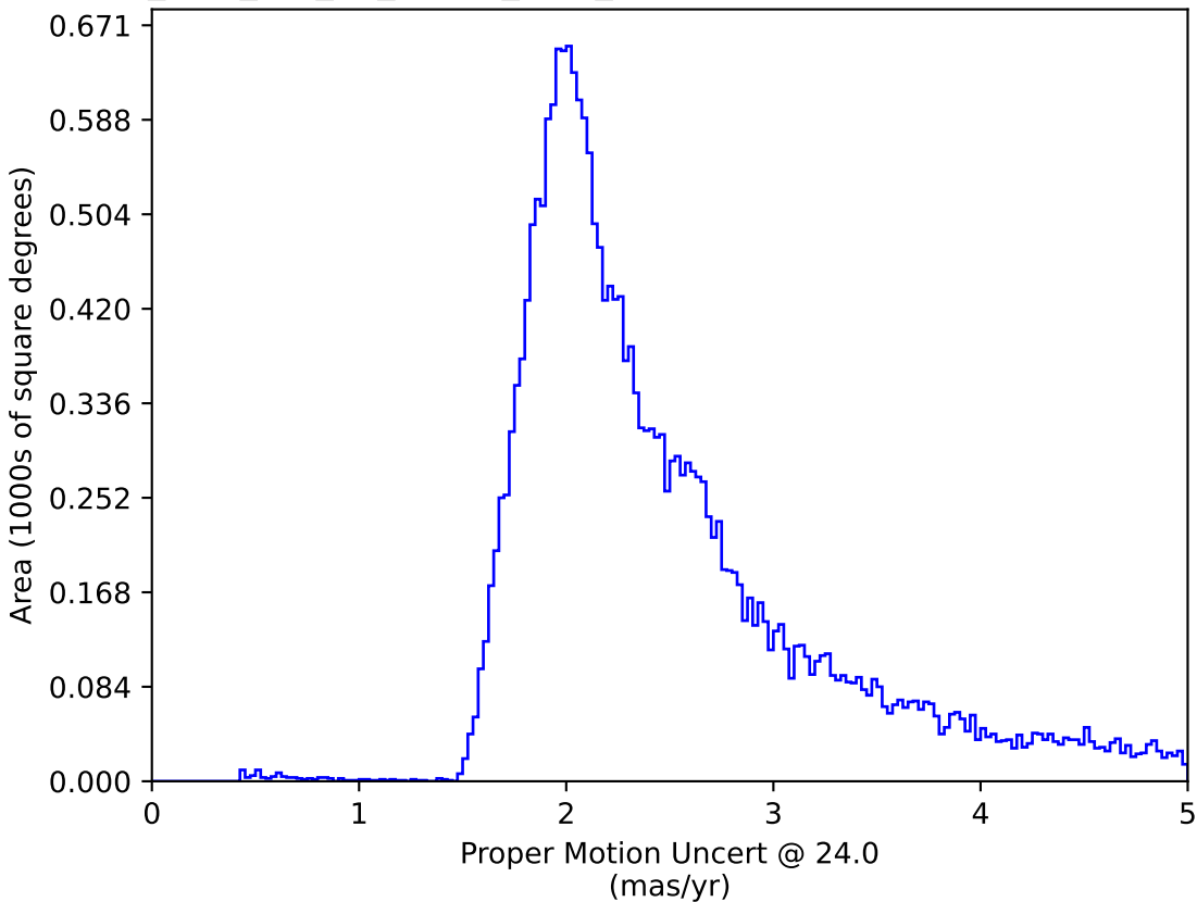
too_elab_r16_d2_ugrizy_v3.4_10yrs : Proper Motion Uncert @ 24.0
