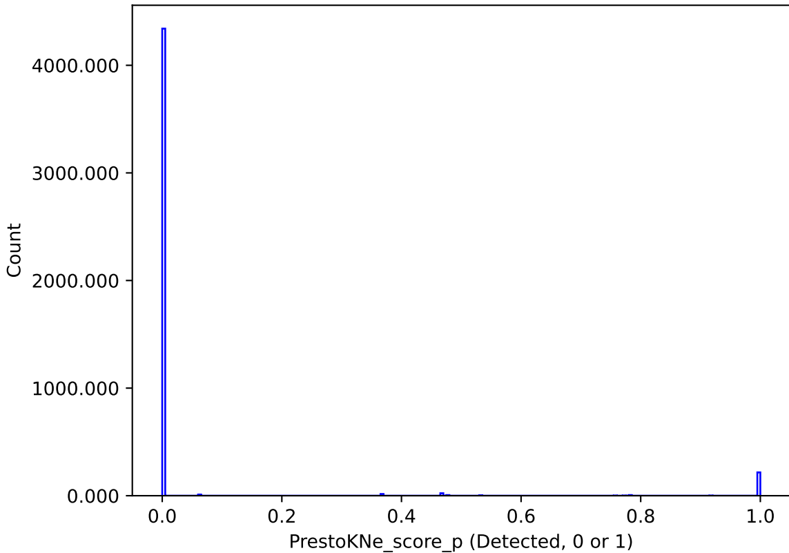
too_elab_r16_d2_ugrizy_v3.4_10yrs : PrestoKNe_score_p
