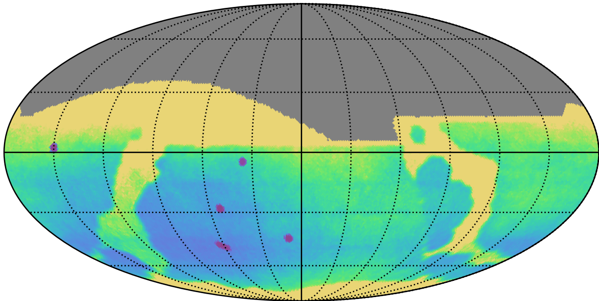
too_elab_r16_d2_ugrizy_v3.4_10yrs : Parallax Uncert @ 24.0
