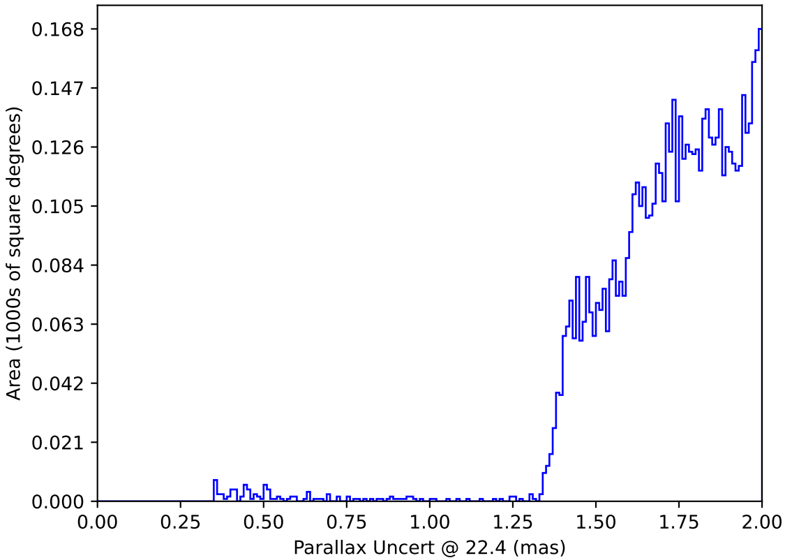
too_elab_r16_d2_ugrizy_v3.4_10yrs : Parallax Uncert @ 22.4
