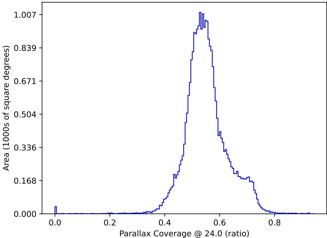
too_elab_r16_d2_ugrizy_v3.4_10yrs : Parallax Coverage @ 24.0
