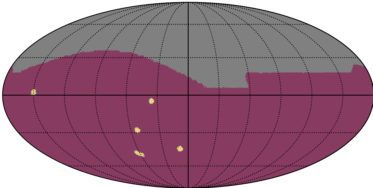
too_elab_r16_d2_ugrizy_v3.4_10yrs : NumberOfQuickRevisits
