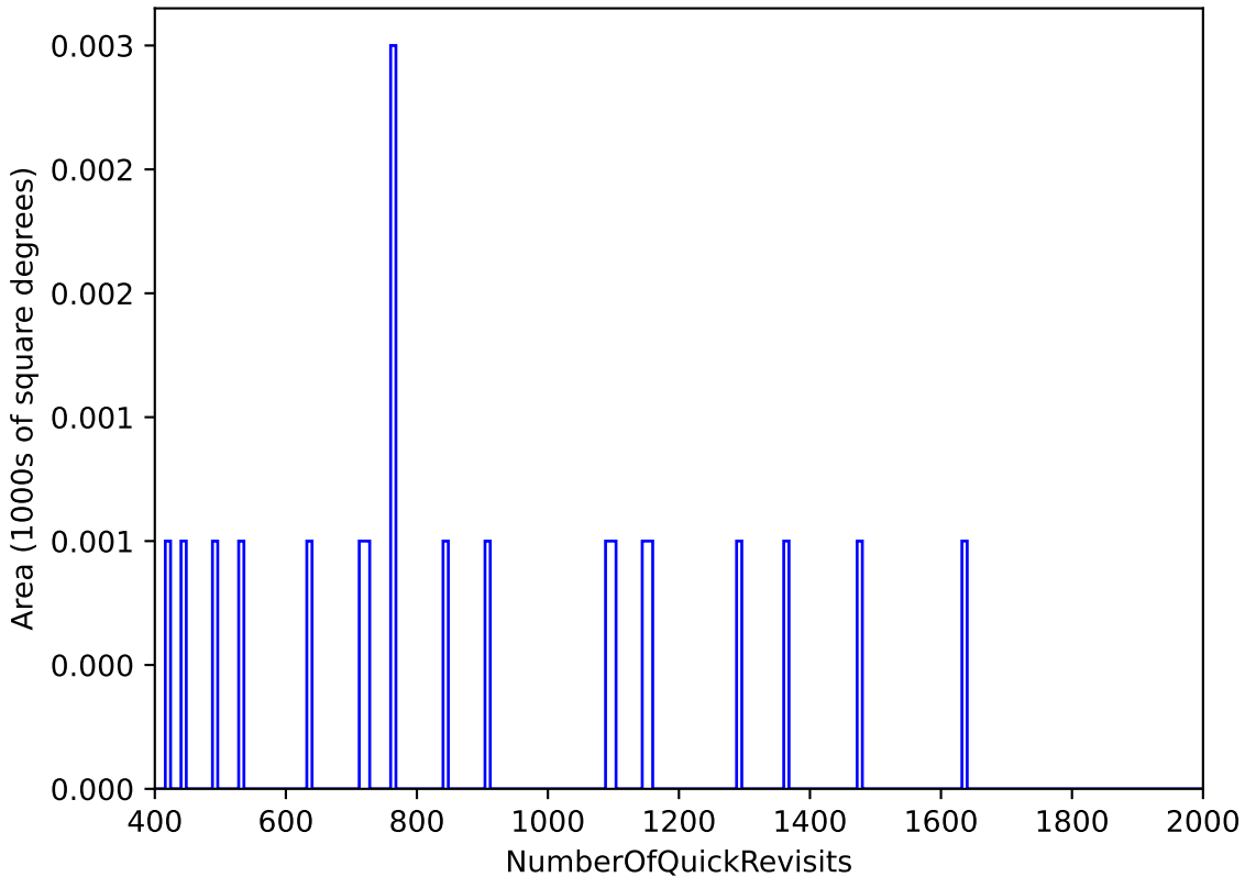
too_elab_r16_d2_ugrizy_v3.4_10yrs : NumberOfQuickRevisits
