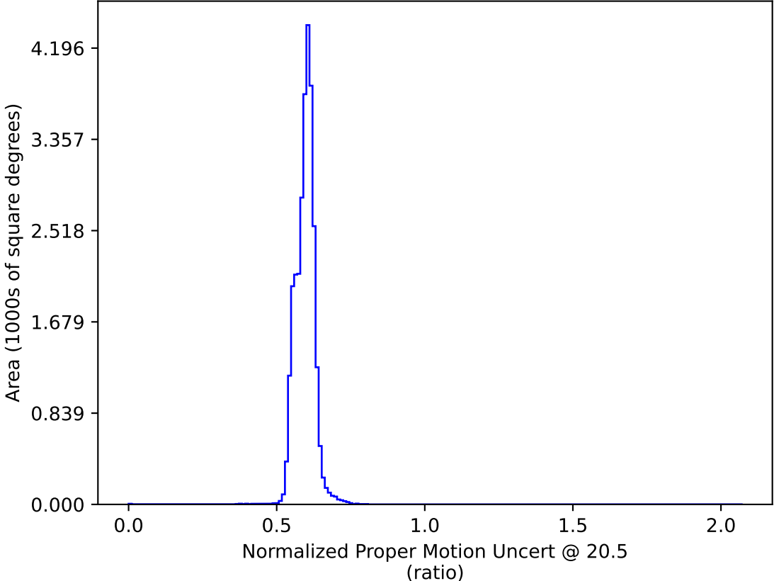
too_elab_r16_d2_ugrizy_v3.4_10yrs : Normalized Proper Motion Uncert @ 20.5
