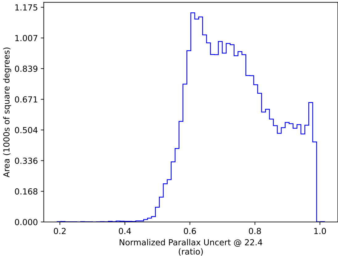
too_elab_r16_d2_ugrizy_v3.4_10yrs : Normalized Parallax Uncert @ 22.4
