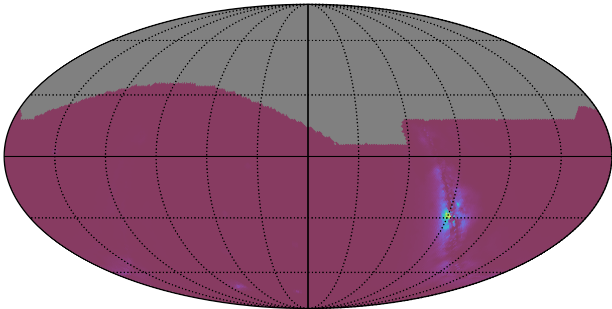
too_elab_r16_d2_ugrizy_v3.4_10yrs : NlcPoints
