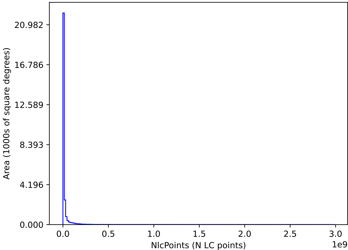
too_elab_r16_d2_ugrizy_v3.4_10yrs : NlcPoints
