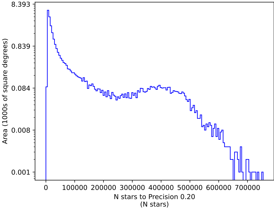
too_elab_r16_d2_ugrizy_v3.4_10yrs z: N stars to Precision 0.20
