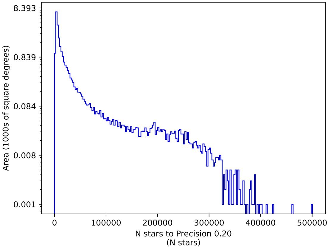
too_elab_r16_d2_ugrizy_v3.4_10yrs u: N stars to Precision 0.20
