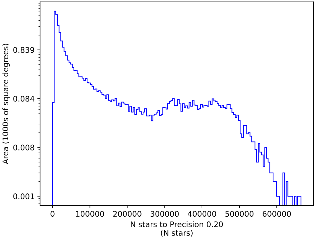
too_elab_r16_d2_ugrizy_v3.4_10yrs r: N stars to Precision 0.20
