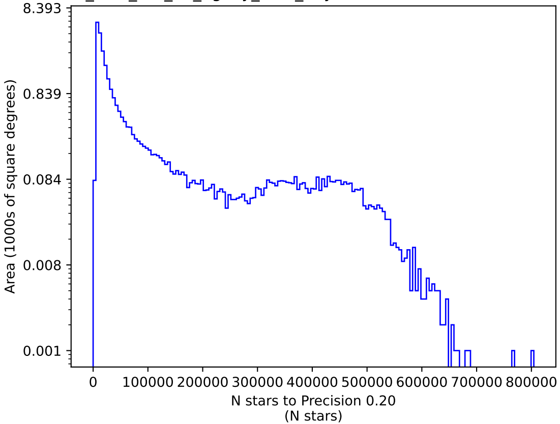
too_elab_r16_d2_ugrizy_v3.4_10yrs i: N stars to Precision 0.20
