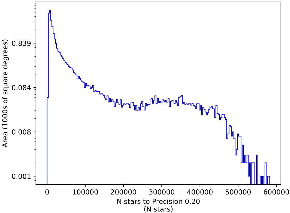
too_elab_r16_d2_ugrizy_v3.4_10yrs g: N stars to Precision 0.20
