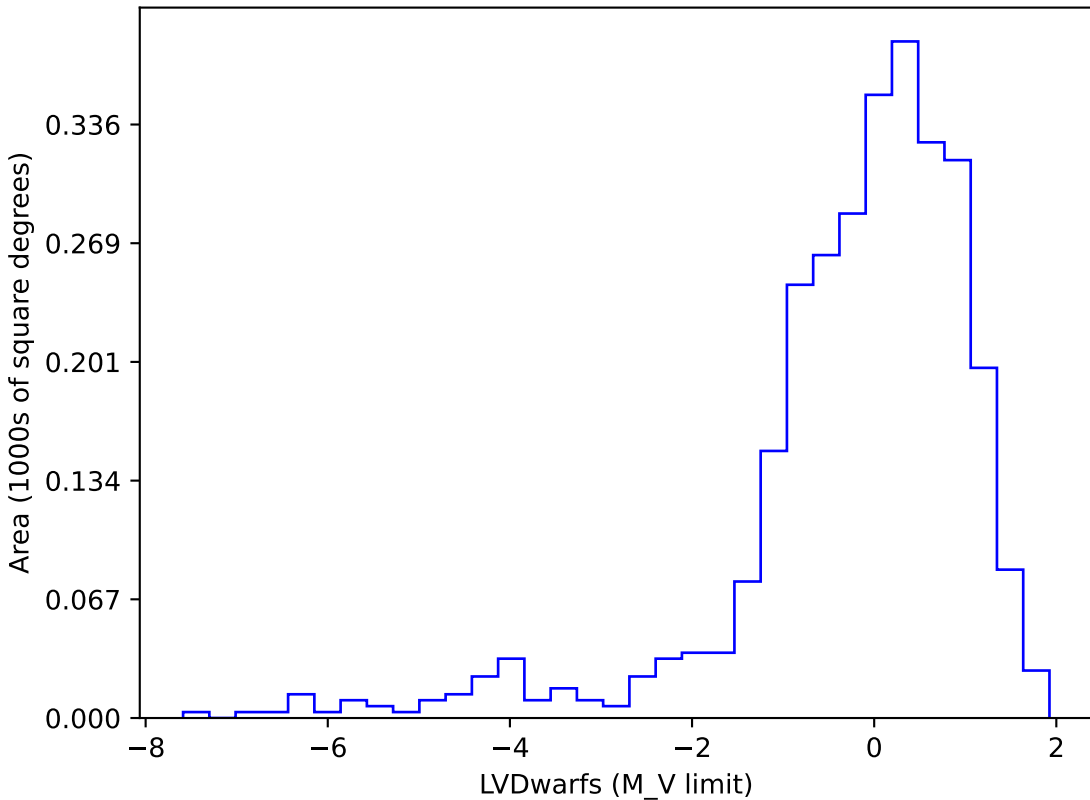
too_elab_r16_d2_ugrizy_v3.4_10yrs gi SCP: LVDwarfs
