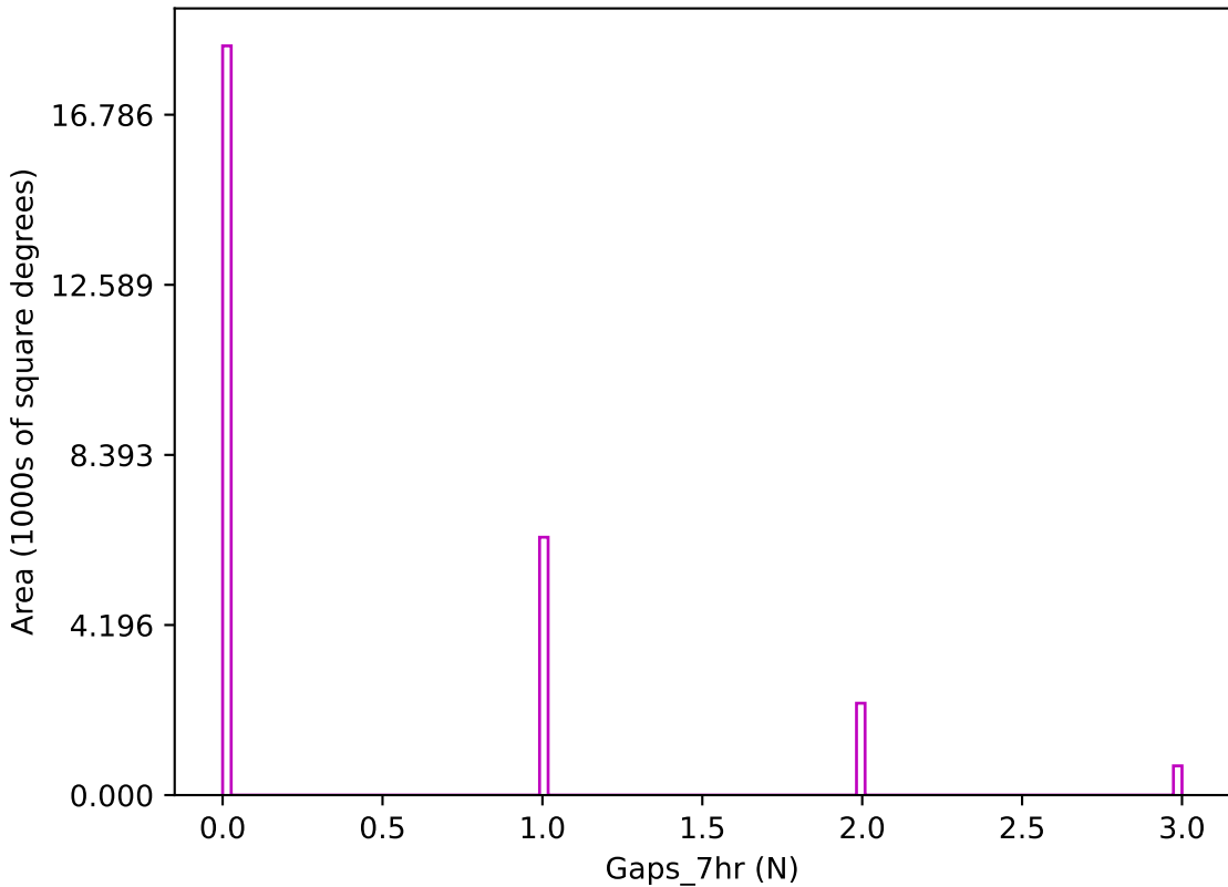
too_elab_r16_d2_ugrizy_v3.4_10yrs z band: Gaps_7hr
