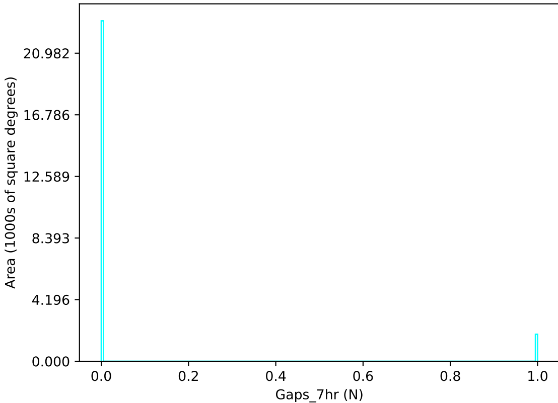
too_elab_r16_d2_ugrizy_v3.4_10yrs u band: Gaps_7hr
