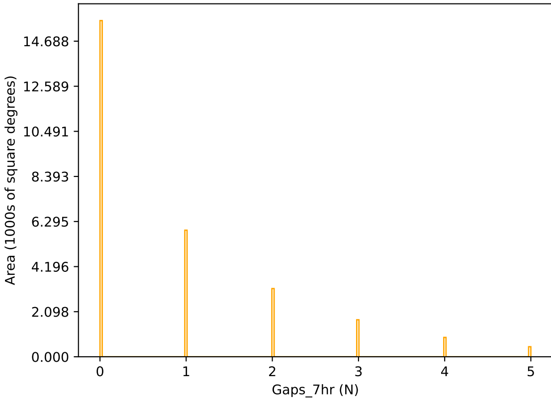
too_elab_r16_d2_ugrizy_v3.4_10yrs r band: Gaps_7hr
