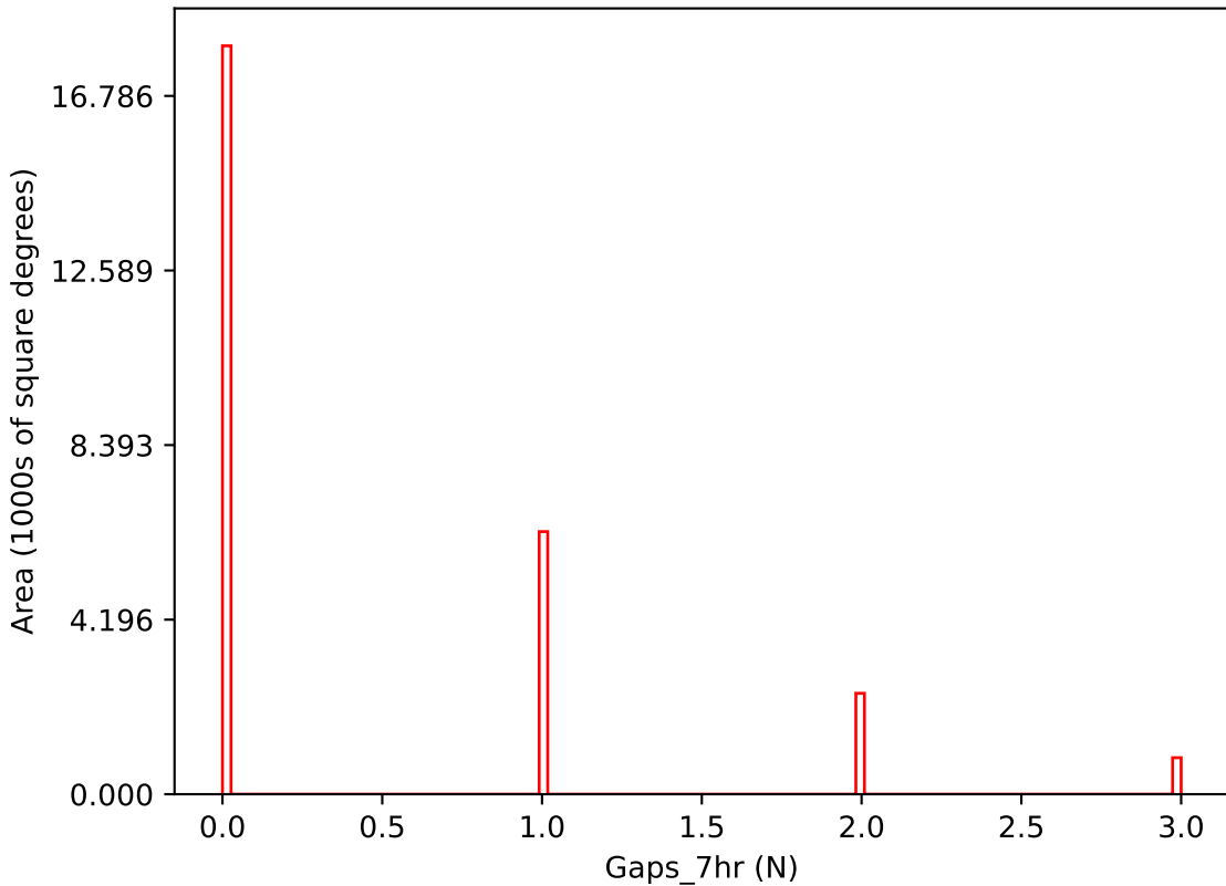
too_elab_r16_d2_ugrizy_v3.4_10yrs i band: Gaps_7hr
