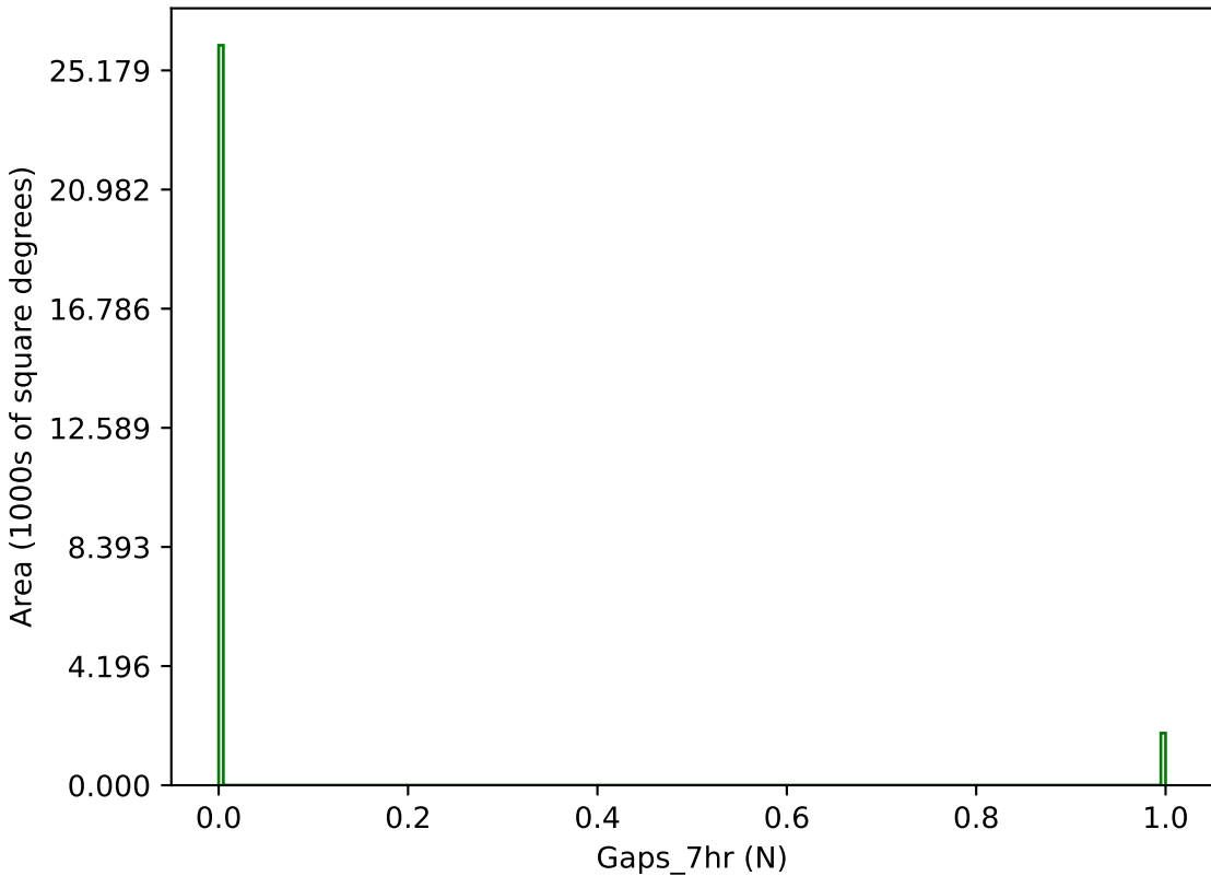
too_elab_r16_d2_ugrizy_v3.4_10yrs g band: Gaps_7hr
