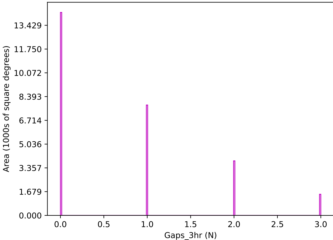
too_elab_r16_d2_ugrizy_v3.4_10yrs z band: Gaps_3hr
