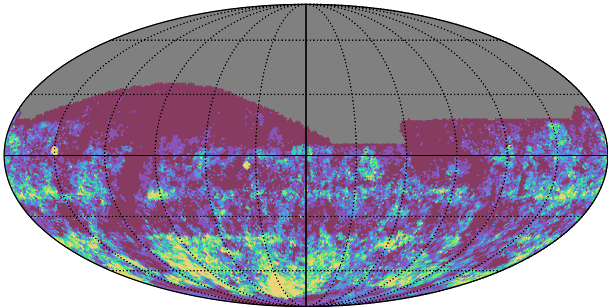
too_elab_r16_d2_ugrizy_v3.4_10yrs r band: Gaps_3hr
