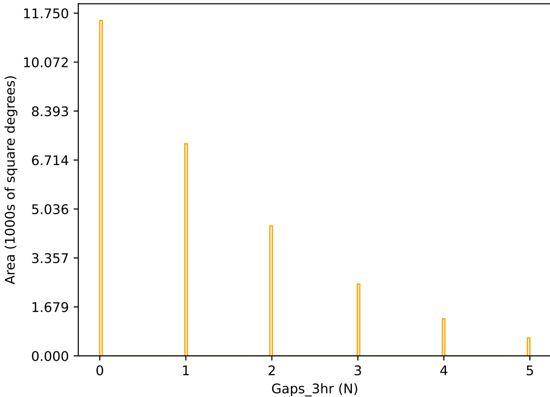
too_elab_r16_d2_ugrizy_v3.4_10yrs r band: Gaps_3hr
