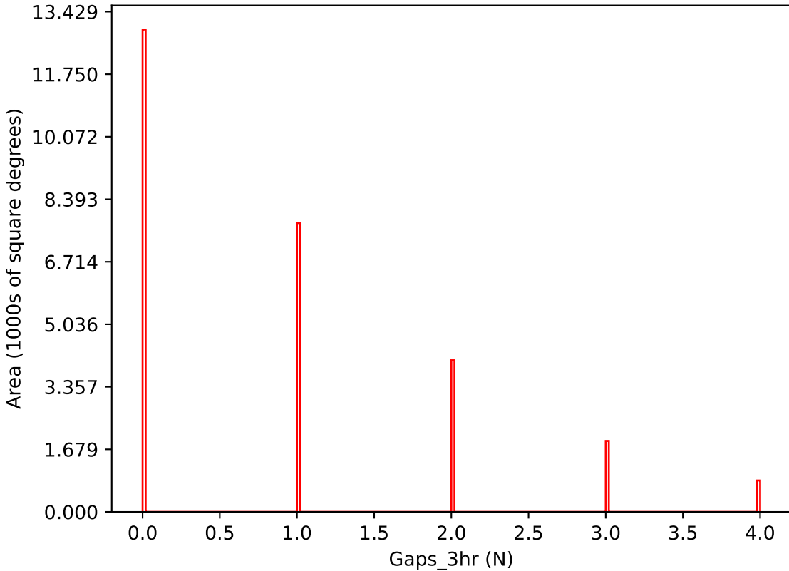
too_elab_r16_d2_ugrizy_v3.4_10yrs i band: Gaps_3hr
