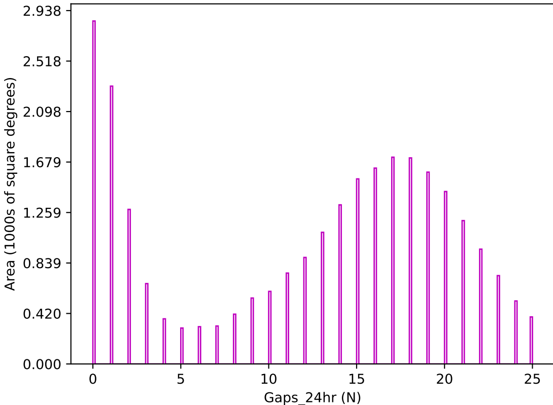
too_elab_r16_d2_ugrizy_v3.4_10yrs z band: Gaps_24hr
