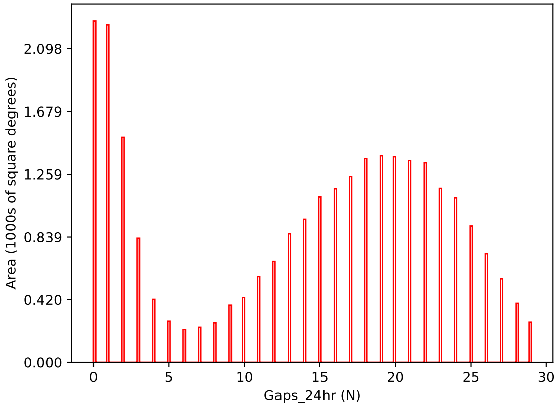
too_elab_r16_d2_ugrizy_v3.4_10yrs i band: Gaps_24hr
