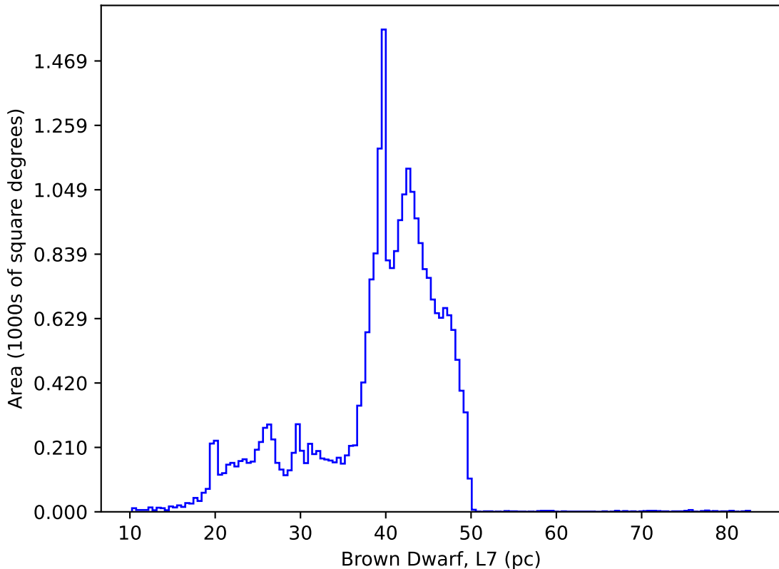
too_elab_r16_d2_ugrizy_v3.4_10yrs : Brown Dwarf, L7
